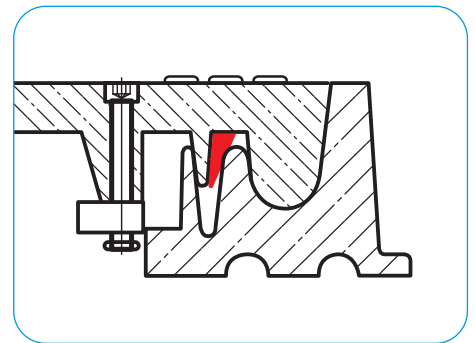
HERMELOCK cover WITH hermetical sealing A
